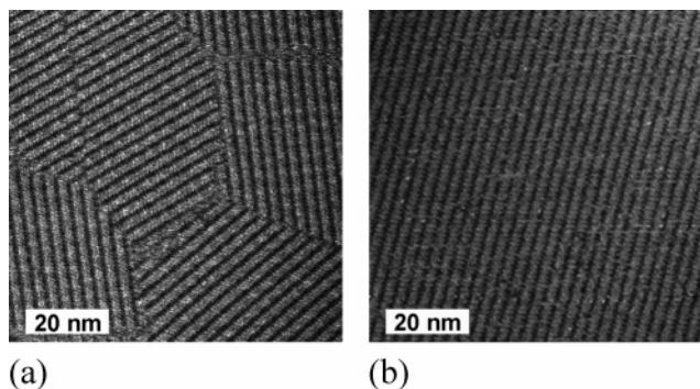
Figure 2. STM image of a monolayer of 3 on HOPG formed (a) from dichloromethane solution ( 80 \text{ nm} \times 80 \text{ nm} , U_b = -700 \text{ mV} , I_t = 8 \text{ pA} ) and (b) from hexane solution ( 80 \text{ nm} \times 80 \text{ nm} , U_b = -700 \text{ mV} , I_t = 10 \text{ pA} ). In image (a), different small domains can be seen; image (b) shows part of a domain extending over more than 500 \text{ nm} \times 500 \text{ nm} .
