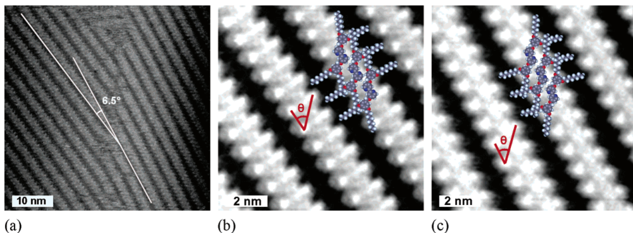
Figure 4. (a) STM images of two domains of monolayers of 3 on HOPG. The angle difference between the two domains is 6.5^\circ . (b) and (c) Expanded images ( 10 \text{ nm} \times 10 \text{ nm} ) of the left and right domains, respectively, of (a). Panel (b) corresponds to conformation anti,anti-3 ( \theta = 55^\circ ), and panel (c) corresponds to conformation anti,syn-3 ( \theta = 38^\circ ) (see Chart 4 and later discussion). Scan parameters: 50 \text{ nm} \times 50 \text{ nm} , U_b = -1111 \text{ mV} , I_t = 15 \text{ pA} .
