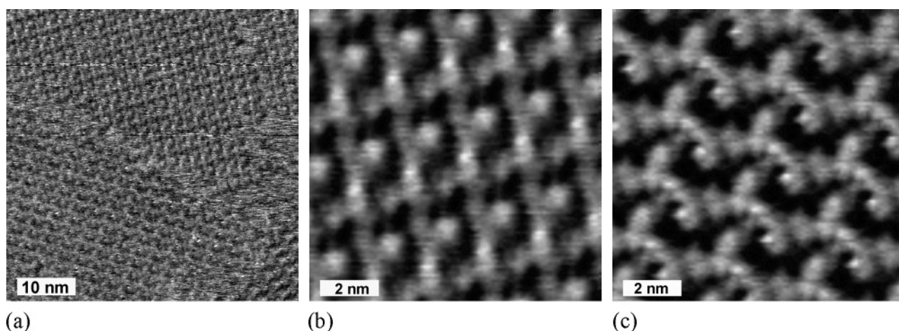
Figure 5. (a) STM images of two domains of monolayers of 6 on HOPG ( 50 \text{ nm} \times 50 \text{ nm} ). (b) and (c) Expanded images ( 10 \text{ nm} \times 10 \text{ nm} ) of the upper and lower domains, respectively, of (a). Scan parameters: U_b = -1111 \text{ mV} , I_t = 15 \text{ pA} .
