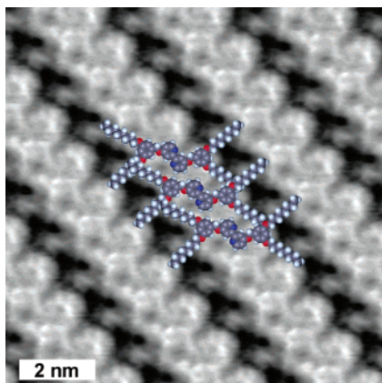
Figure 3. STM image of a monolayer of 3 formed from hexane solution on HOPG ( 10 \text{ nm} \times 10 \text{ nm} , averaged over 41 positions, U_b = -900 \text{ mV} , I_t = 40 \text{ pA} ). The benzyl groups have the highest intensity. Molecular models of 3 showing the best-fit conformation are also shown; this is discussed later in the article.
